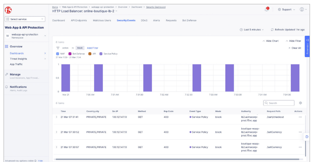
Figure 4: Protected API endpoint where request is returning 403 response code to client(s) who are not authorized to access.
