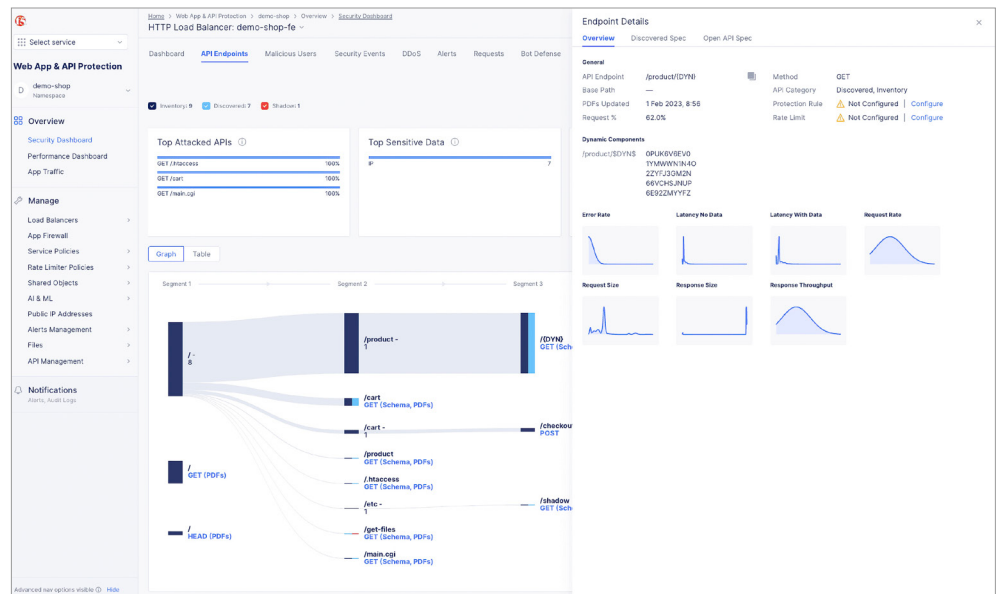
Figure 7: Endpoint details include metrics such as request size and response size, latency with and without data, request rate and error rate, and response throughput.
